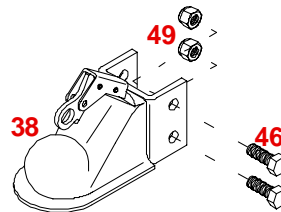
2-5/16" Lever Lock Bolt On Coupler RATED AT 7500#
